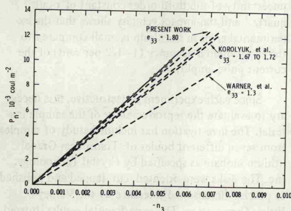
FIG. 1. The experimentally observed piezoelectric polarization is plotted at various compressive Lagrangian strains. The various dashed lines represent extrapolations to large strain of the linear piezoelectric constant, e_{33} , observed by various authors.
